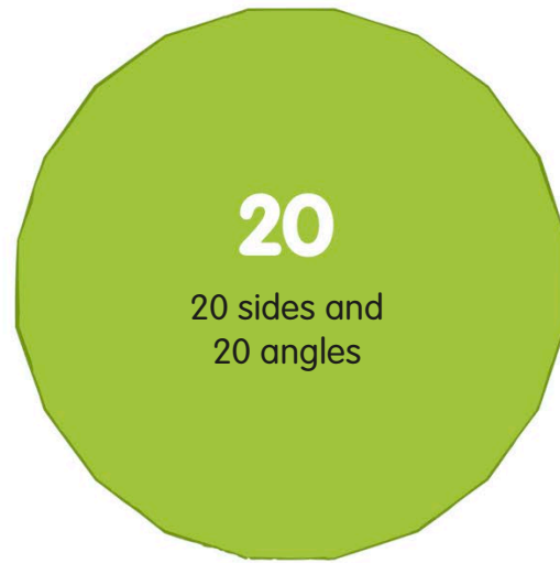
Regular icosagon
