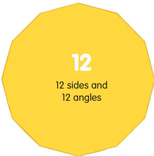
Regular dodecagon
