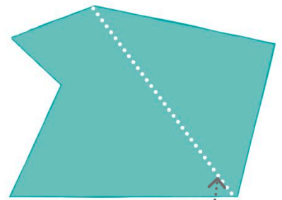
Diagonal
