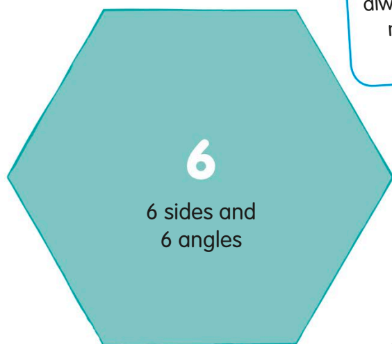
Regular hexagon
