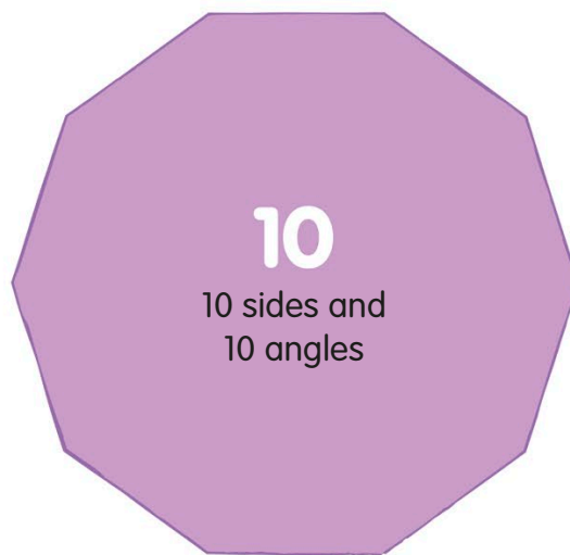
Regular decagon
