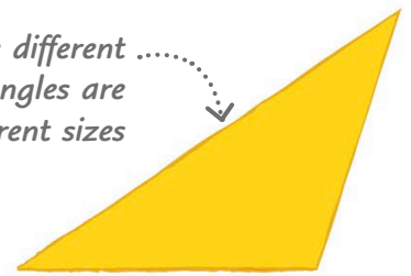
Irregular triangle
