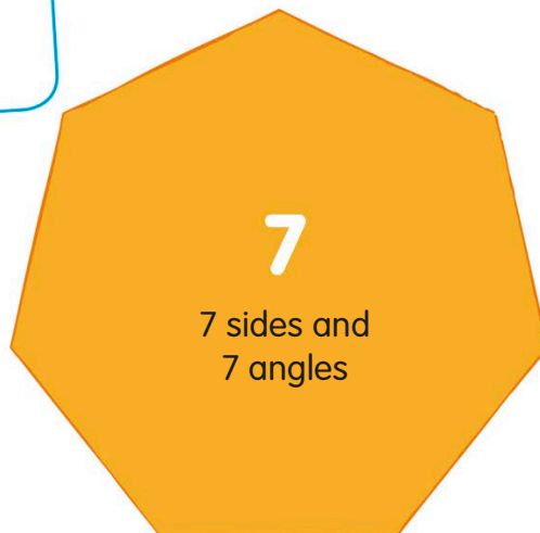
Regular heptagon
