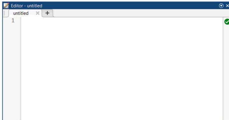
Fig.9.15 MATLAB Editor
