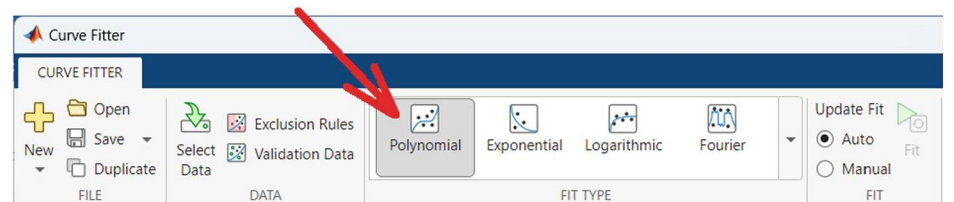
Fig.6.16 Polynomial regression
