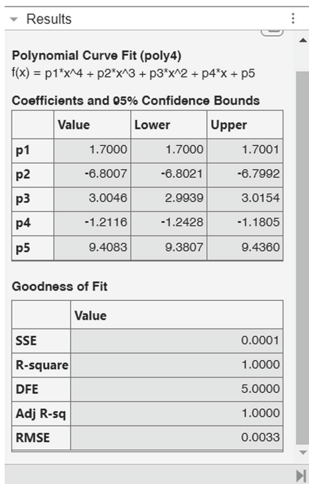
Fig. 6.23 Calculated coefficients
