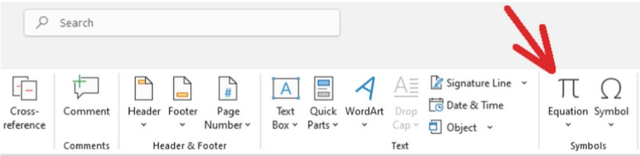
Fig. 14.3 Equations button
