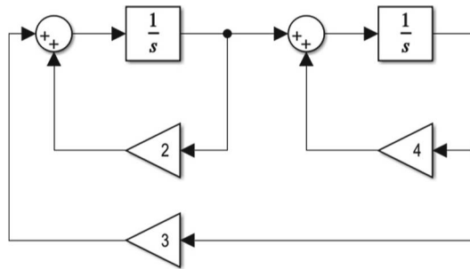
Fig. 12.18 Simulink model with updated gains
