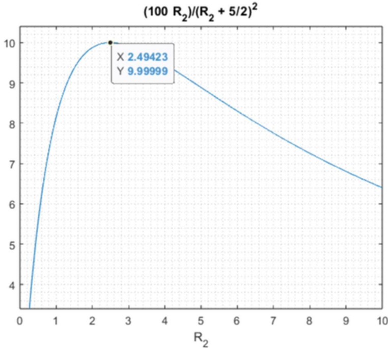
Fig. 1.42 The function P_{R_2} = \frac{100R_2}{(2.5+R_2)^2} reaches its peak value of 10 around the point 2.5 on the x-axis
