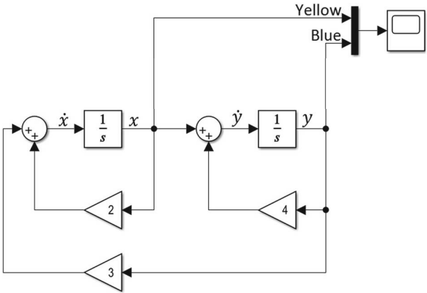
Fig. 12.23 The left and right integrators output x(t) and y(t) , respectively
