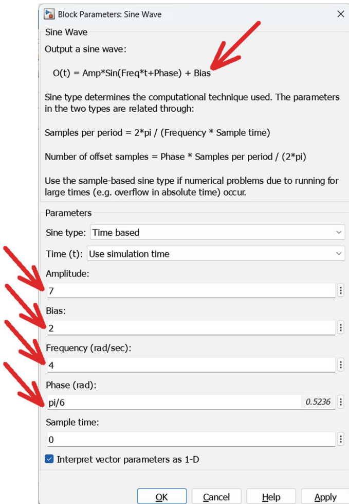
Fig. 12.51 Required settings to generate u(t) = 2 + 7\sin(4t + \frac{\pi}{6})
