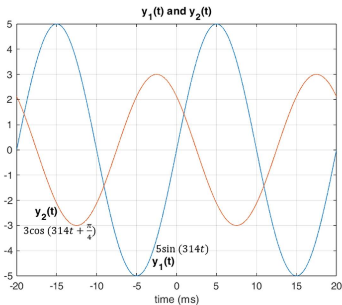
Fig. 2.9 Plot of y_1(t) = 5\sin(314t) and y_2(t) = 3\cos\left(314t + \frac{\pi}{4}\right)
