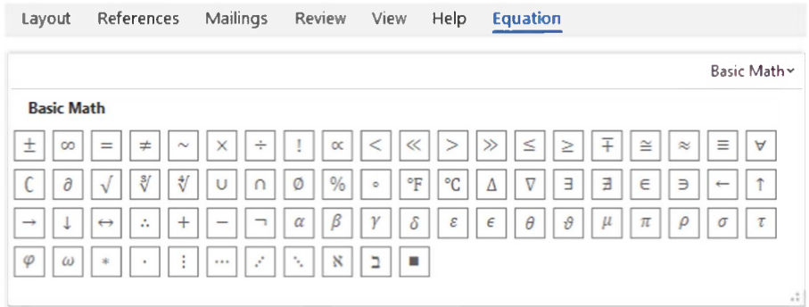
Fig. 14.7 Opened window
