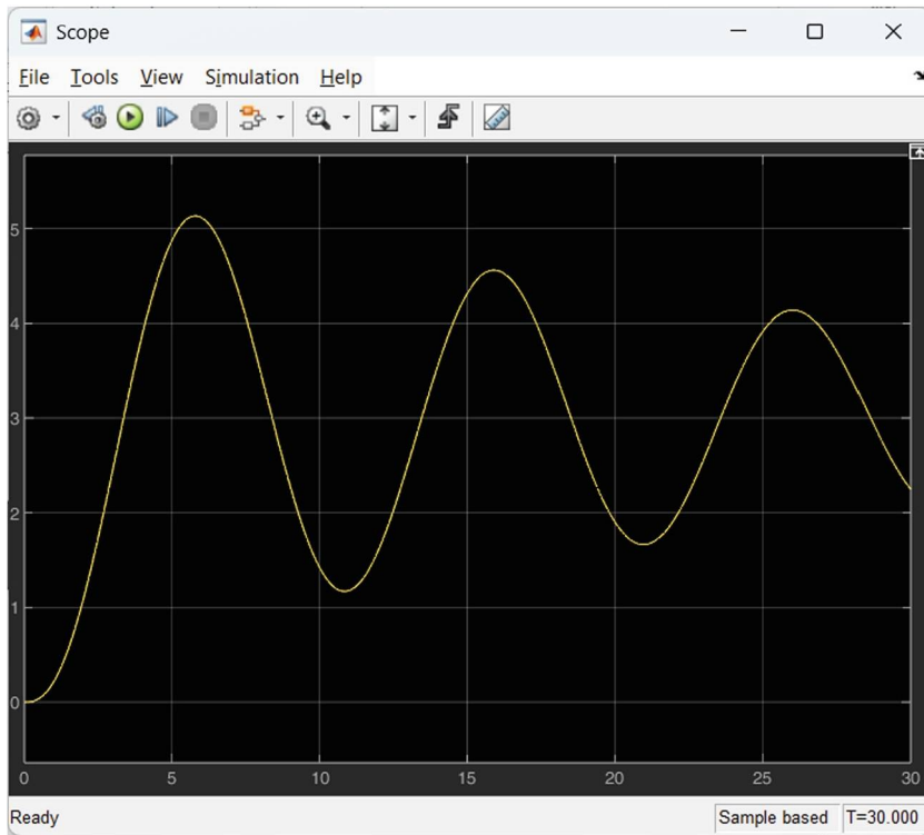
Fig. 12.65 Simulation results
