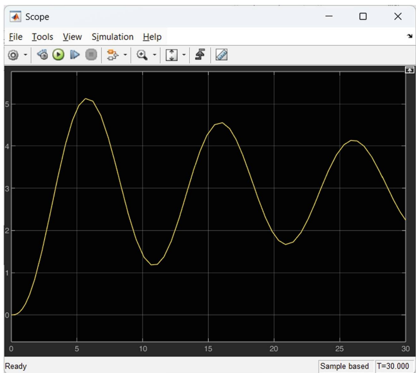
Fig. 12.61 Simulation results
