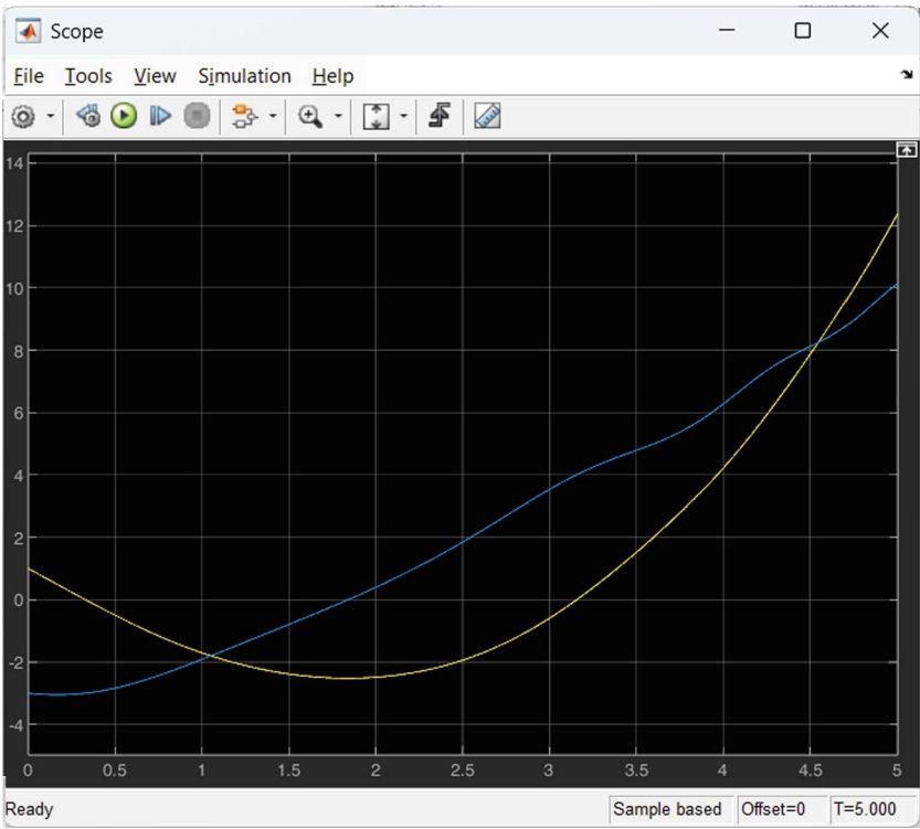
Fig. 12.79 Simulation results
