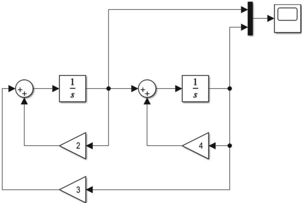
Fig. 12.21 A multiplexer and scope block are added to the model
