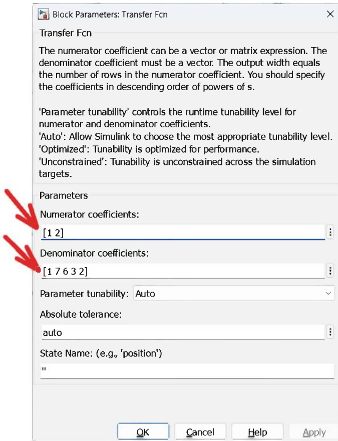
Fig. 12.58 Required settings to define T(s) = \frac{Y(s)}{X(s)} = \frac{s+2}{s^4+7s^3+6s^2+3s+2}
