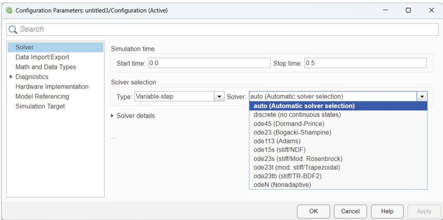
Fig. 12.27 Supported solvers
