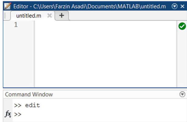
Fig. 9.51 MATLAB Editor
