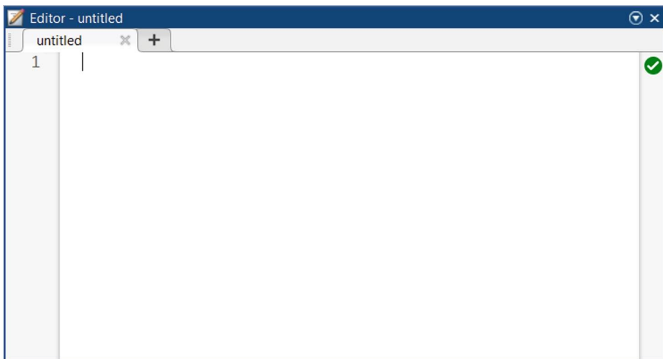
Fig. 1.75 Editor window
