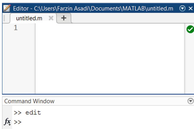
Fig. 5.6 MATLAB editor
