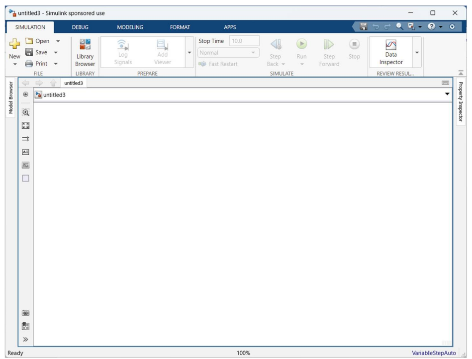
Fig. 12.4 Simulink environment
